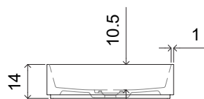
versione marmo CUBA01 Marble Product CUBA01
