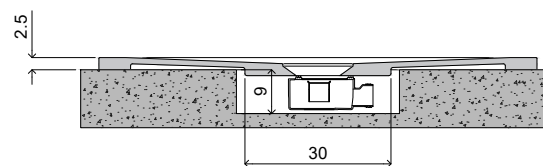
Versione appoggio Surface-mounted version
